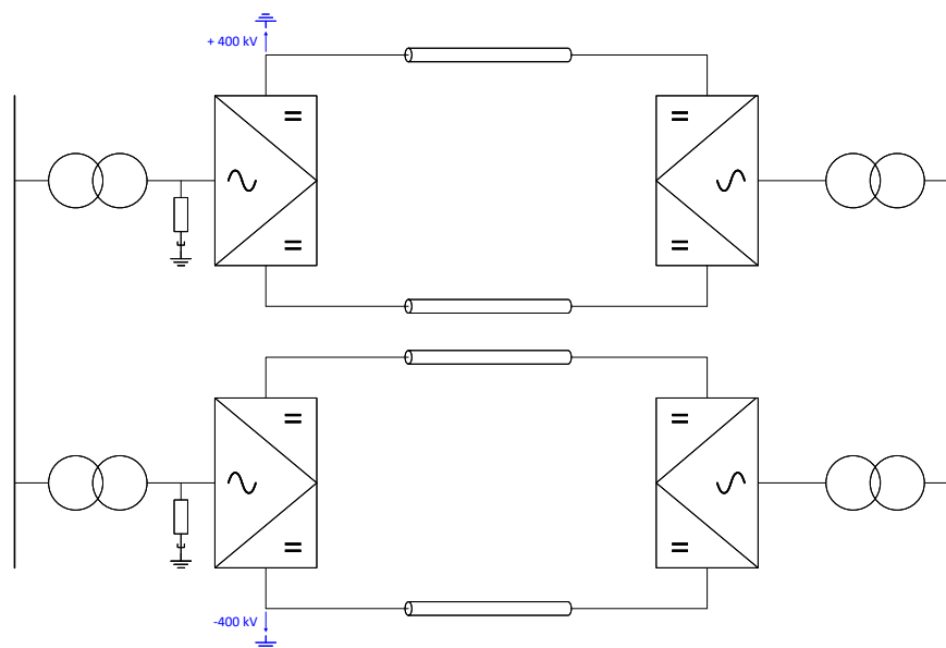
Figure 3: Dual symmetrical monopole (DSMP) configuration.
